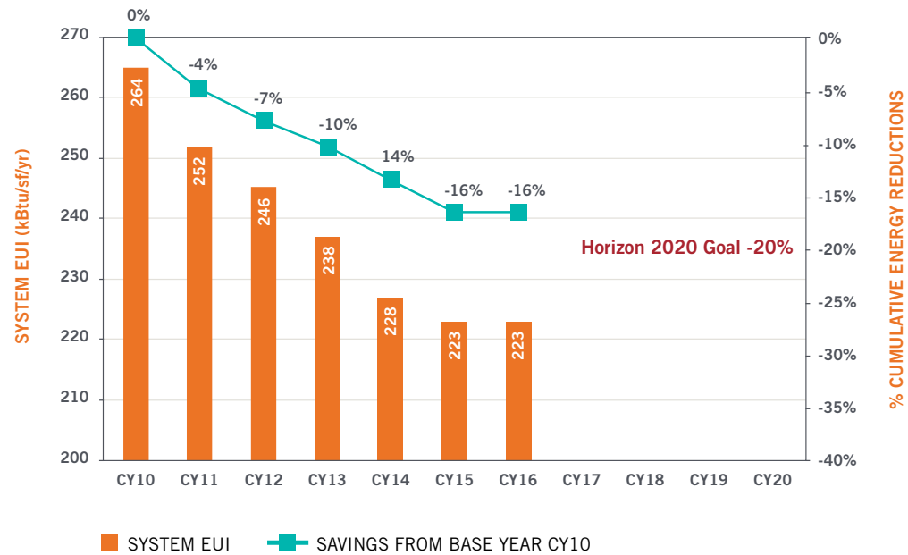
System Energy Use Intensity and % Cumulative Reductions
